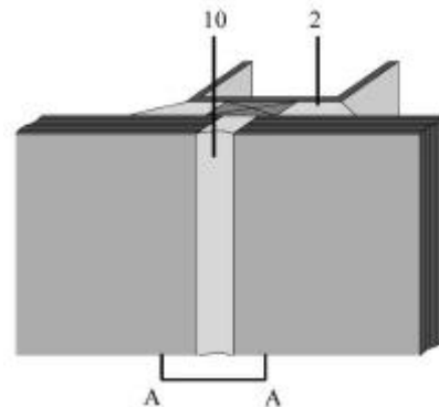
Figure 3B: A mullion detail.
